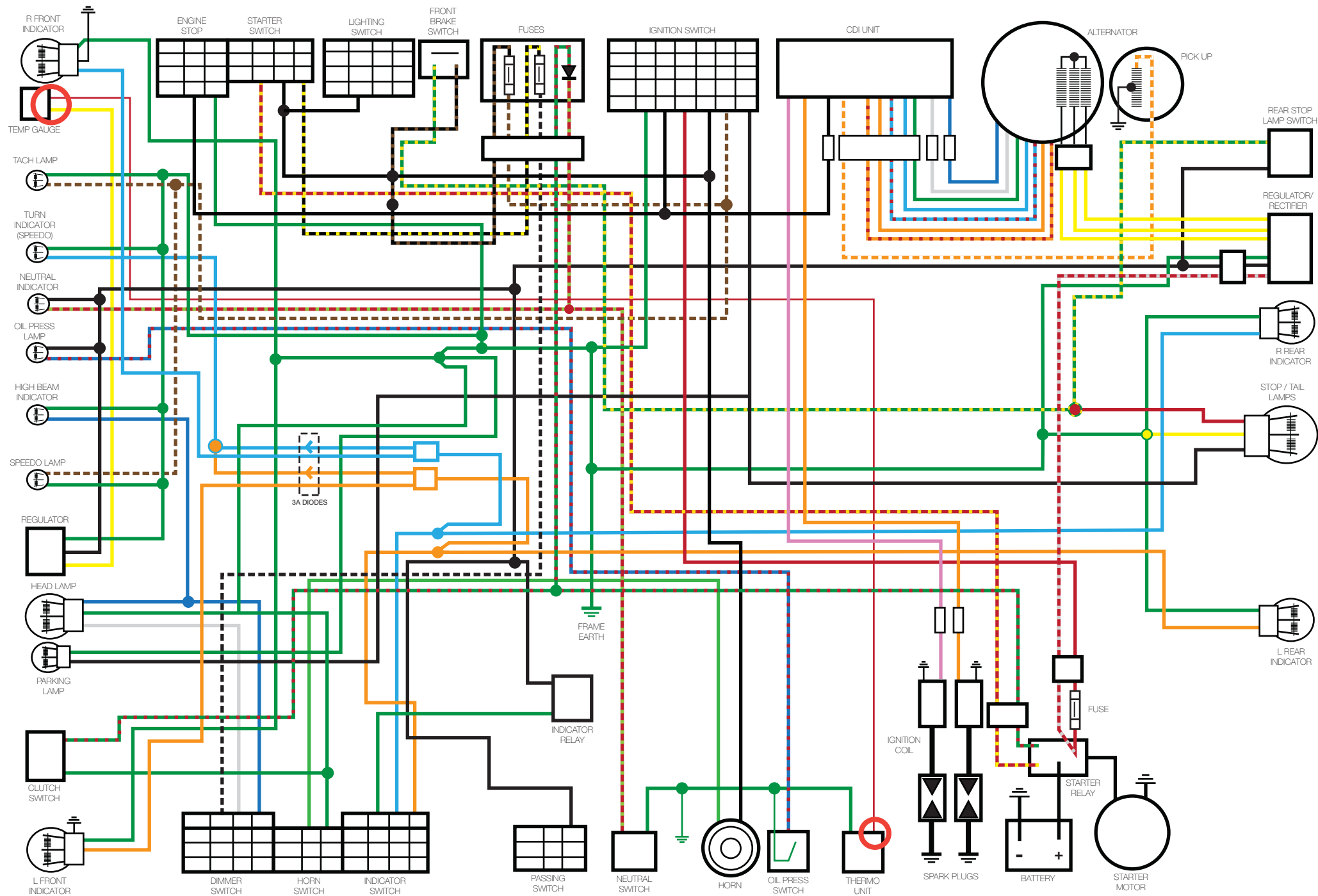
PERSONAL WIRING DIAGRAM 1981 HONDA CX500-B
